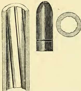
The Henry Rifling and Bullet, and Regulation Pattern Cartridge.
